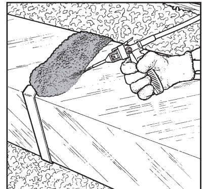
Figure 5: Duct joint sealing (ignition barrier required)
