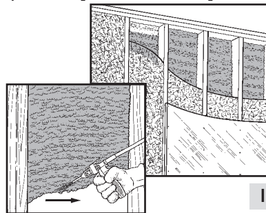
Figure 7: Flash and batt (1/2"-1" [13 mm-25 mm] thickness)
