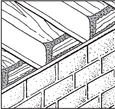
Figure 9: Sealing sill plate/rim joists (maximum 2" [50 mm] thickness)
