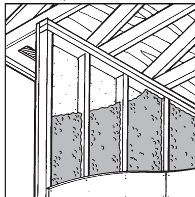
Figure 8: Insulating stud wall cavities (maximum 2" [50 mm] thickness)
